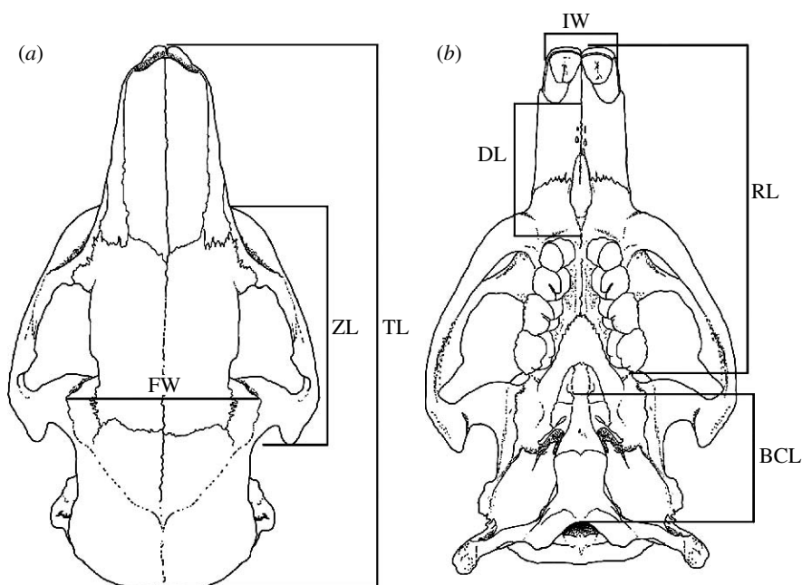
Figure 4. Skull of Myocastor coypus in (a) dorsal view and (b) ventral view showing the skull variables used for allometric analysis. RL, rostral length; DL, diastema length; BCL, basicranial length (basioccipital + basisphenoid); IW, incisors width; ZL, zygomatic arch length; FW, frontal width; TL, total length.
