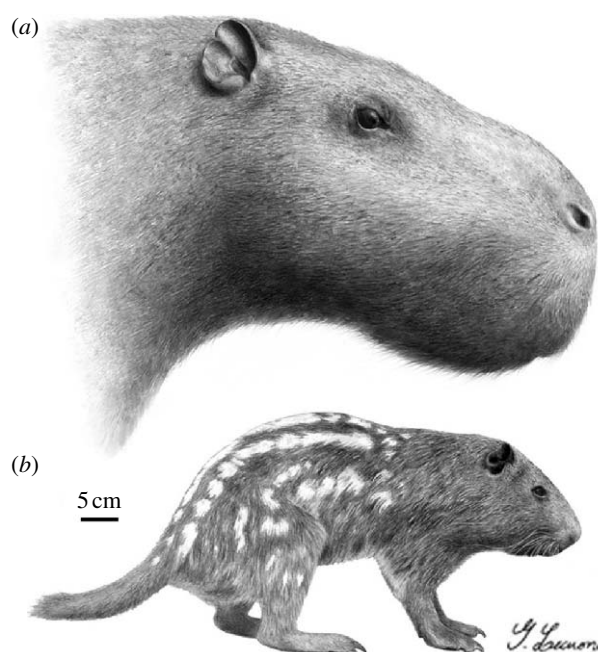
Figure 3. Reconstruction of the head of (a) J. monesi in comparison with (b) the living pakarana ( D. branickii ).
