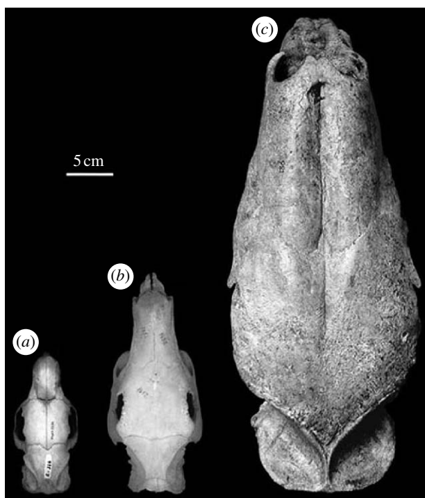
Figure 2. Skulls (dorsal view) of (a) D. branickii , (b) H. hydrochaeris and (c) J. monesi .
