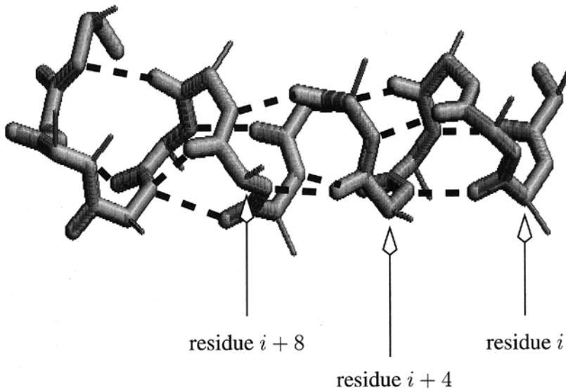
Figure 1.13 An \alpha helix. The stabilizing hydrogen bonds are shown with dashed lines.
