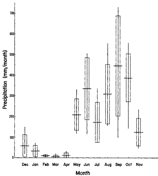
FIGURE 4. Monthly precipitation at La Asunción on Volcán Mombacho (elev. 580 m). The data span a four year period from December 1972 to November 1976. The vertical bars, horizontal bars, and rectangles represent the range, mean, and one standard deviation from the mean respectively (data provided by Empresa Nacional de Luz y Fuerza).
