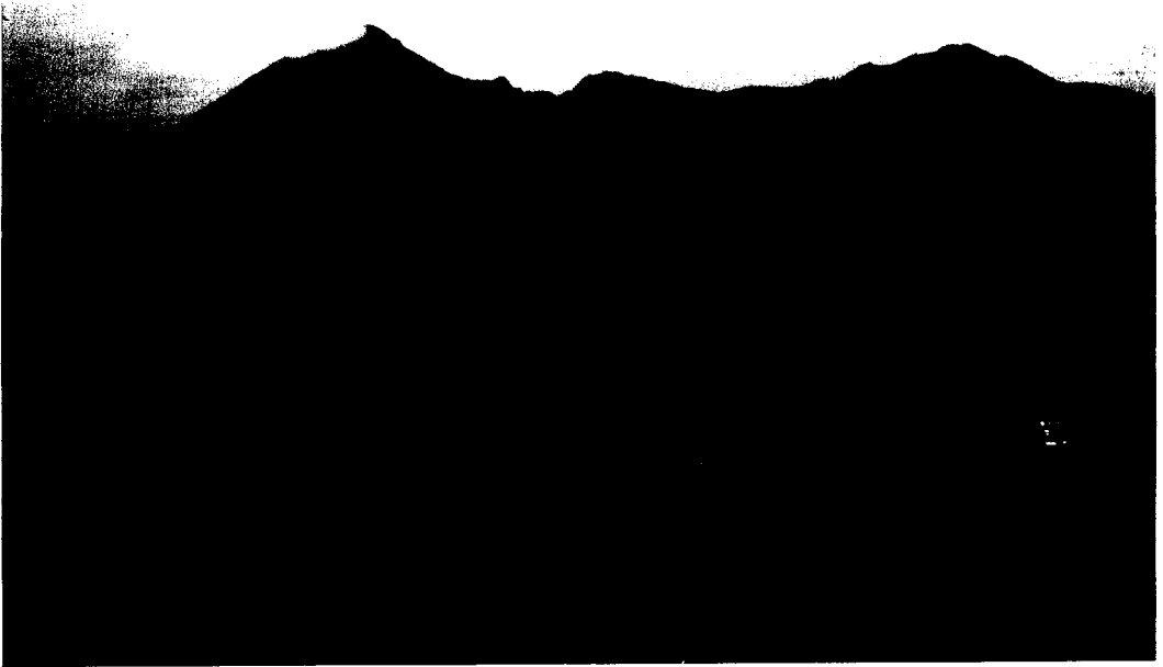
FIGURE 1. Profile view of Mombacho from the north.
