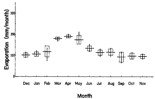
FIGURE 5. Monthly evaporation at La Asunción on Volcán Mombacho (elev. 580 m). The data span a four year period from December 1972 to November 1976. The vertical bars, horizontal bars, and rectangles represent the range, mean, and one standard deviation from the mean respectively (data provided by Empresa Nacional de Luz y Fuerza).
